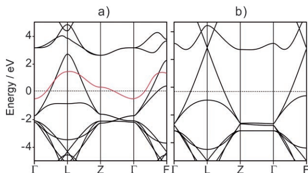
Figure 3. Extended Hückel band structures of \text{CaC}_6 calculated from our optimized parameters. a) With inclusion of Ca 3d states and b) without inclusion of Ca 3d states.
